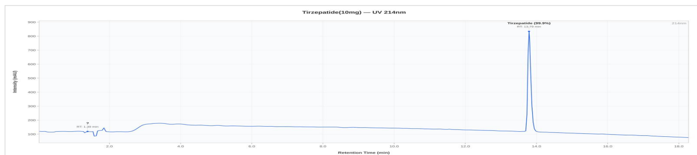
Tirzepatide 10mg - TP-TIRZ10-260614-010: UV Chromatogram
