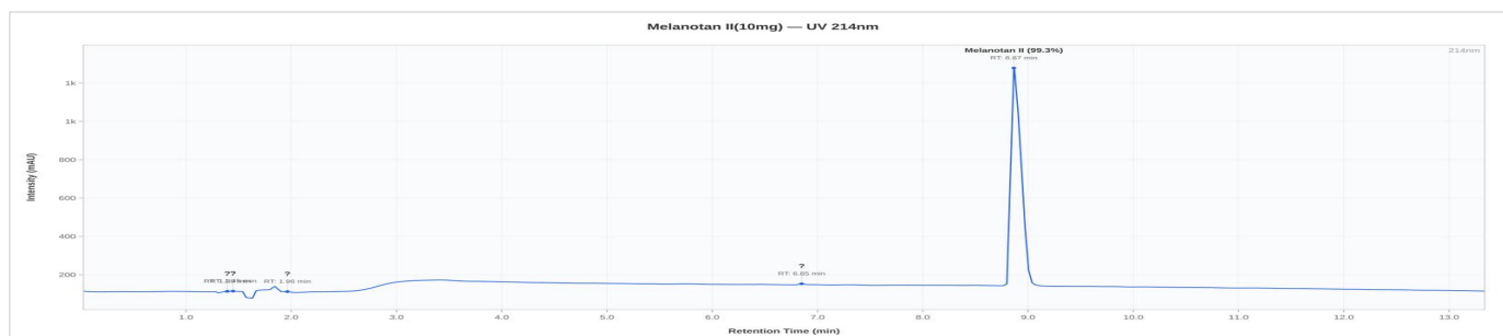
Melanotan II 10mg - TP-MT210-260614-014 : UV Chromatogram
